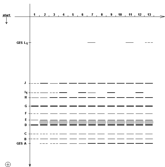
Figure 1. Scheme of the esterase spectra of silkworm gut in PAGE: 1, 2 – 1 st larval instar; 3, 4 – 2 nd larval instar; 5, 6 – 3 rd larval instar; 7-9 – 4 th larval instar; 10-13 – 5 th larval instar; 2, 4, 6 – mixed probes; 1, 3, 5, 7-13 – individual probes.
