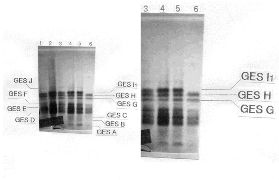
Figure 4. Esterase spectra of silkworm gut in 6.5% PAGE, 4 th larval instar (6) and 5 th larval instar (1÷5): 1 - breed P15; 2, 3 - breed M1; 4, 5 - breed M2; 6 - breed T106.
