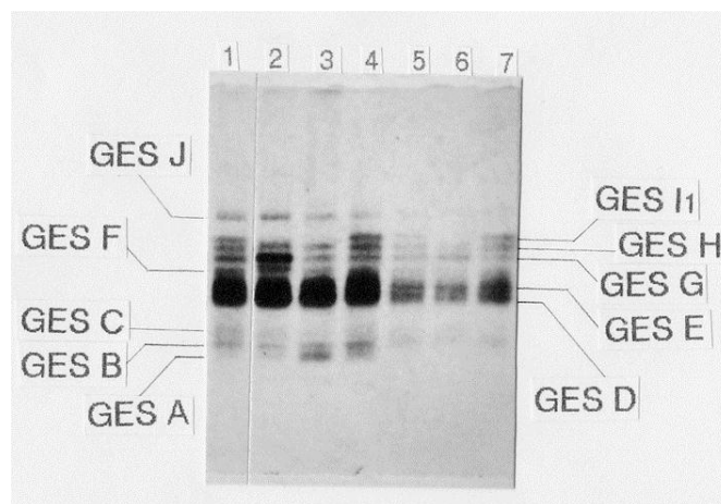
Figure 2. Esterase spectra of silkworm gut in 7.5% PAGE, 1 st larval instar: 1 – breed P15; 2 - breed T108; 3 - breed T106; 4, 7 - breed M2; 5 - hybrid P15xP14; 6 - breed B517; 1-4 - mixed probes, 5-7 - individual probes.
