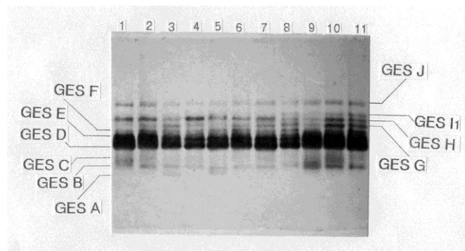
Figure 3. Esterase spectra of silkworm gut in 7.5% PAGE, 2 nd larval instar: 1, 2 - breed UK20; 3-7 - breed Tashkent 16; 8-11 - breed M2; individual probes only.
