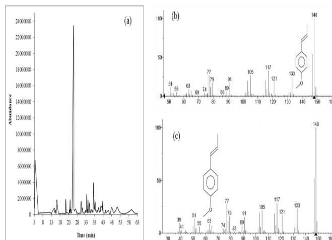
Figure 2. (a) GC-MS chromatogram of Scutellaria orientalis L. subsp. virens (Kotchy & Boiss.) J. R. Edm. essential oil, (b, c) mass spectrum of trans -anethole.
