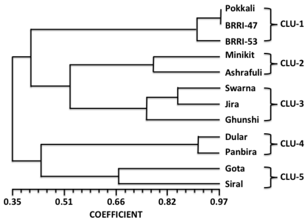
Figure 2. An UPGMA cluster dendrogram showing the genetic relationships of the 12 rice cultivars tested using five RAPD primers. CLU- cluster.
