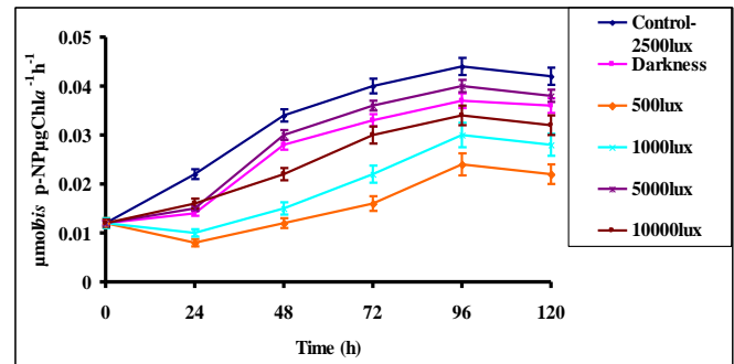
Figure 9B. Effect of different light intensity on phosphodiesterase activity of Leptolyngbya . Temperature 25^{\circ}\text{C} \pm 2^{\circ}\text{C} , pH- 8 (results mean \pm SD N=3 ).
