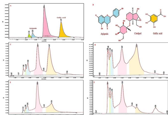
Figure 9. HPLC chromatograms of (A) apigenin, catalpol and gallic acid standards (2.5, 100 and 5 \mu\text{g}\cdot\text{mL}^{-1} ); (B) structure of apigenin, catalpol and gallic acid; (C) aerial part of wild P. lanceolata ; (D) Root part of wild P. lanceolata ; (E) hairy root-derived plantlets; (F) Hairy root of P. lanceolata . R^2 values were y_{\text{Apigenin}} = 296784x + 13686 ; y_{\text{Catalpol}} = 11865x + 4919.9 and y_{\text{Gallic acid}} = 355517x + 24027 . The amount of apigenin, catalpol and gallic acid was also evaluated in aerial and root parts of wild P. lanceolata .
