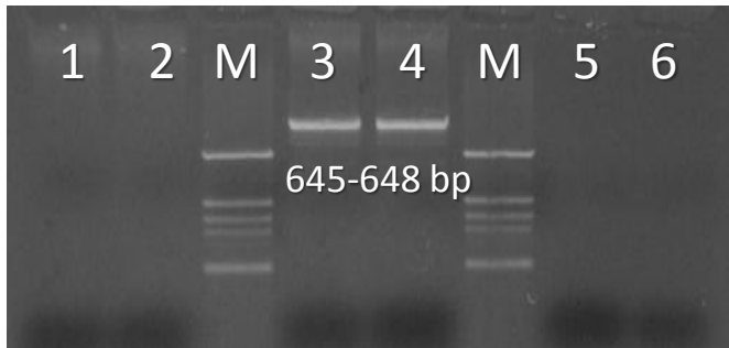
Figure 3. SS_MTDI primer pair cross testing with human, pig and chicken DNA extracted from white blood cells. Lanes 1 and 2 are human DNA, lanes 3 and 4 are pig DNA, lanes 5 and 6 are chicken DNA and lane M is DNA marker with 114, 176, 203, 245 and 500 bp DNA fragments.
