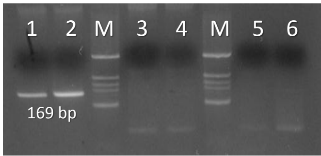
Figure 2. HS_MTDI primer pair cross testing with human, pig and chicken DNA extracted from white blood cells. Lanes 1 and 2 are human DNA, lanes 3 and 4 are pig DNA, lanes 5 and 6 are chicken DNA and lane M is DNA marker with 114, 176, 203, 245 and 500 bp DNA fragments.
