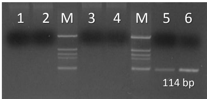
Figure 4. GG_MTDI primer pair cross testing with human, pig and chicken DNA extracted from white blood cells. Lanes 1 and 2 are human DNA, lanes 3 and 4 are pig DNA, lanes 5 and 6 are chicken DNA and lane M is DNA marker with 114, 176, 203, 245 and 500 bp DNA fragments.
