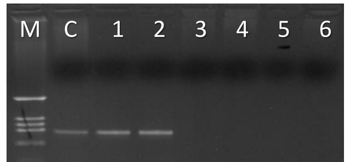
Figure 5. Amplification of DNA extracted from functional cell models with HS_MTDI primer pair. Lane M is DNA marker with 114, 176, 203, 245 and 500 bp DNA fragments, lane C is positive control (human DNA extracted from venous blood). Lane 1 is DNA extracted from functional cell model with UH cell line, lane 2 is DNA extracted from functional cell model with BH cell line, lane 3 is DNA extracted from functional cell model with PSI cell line, lane 4 is DNA extracted from functional cell model with CLAB cell line, lane 5 is DNA extracted from functional cell model with C2 cell line and lane 6 is DNA extracted from functional cell model with PTC cell line.
