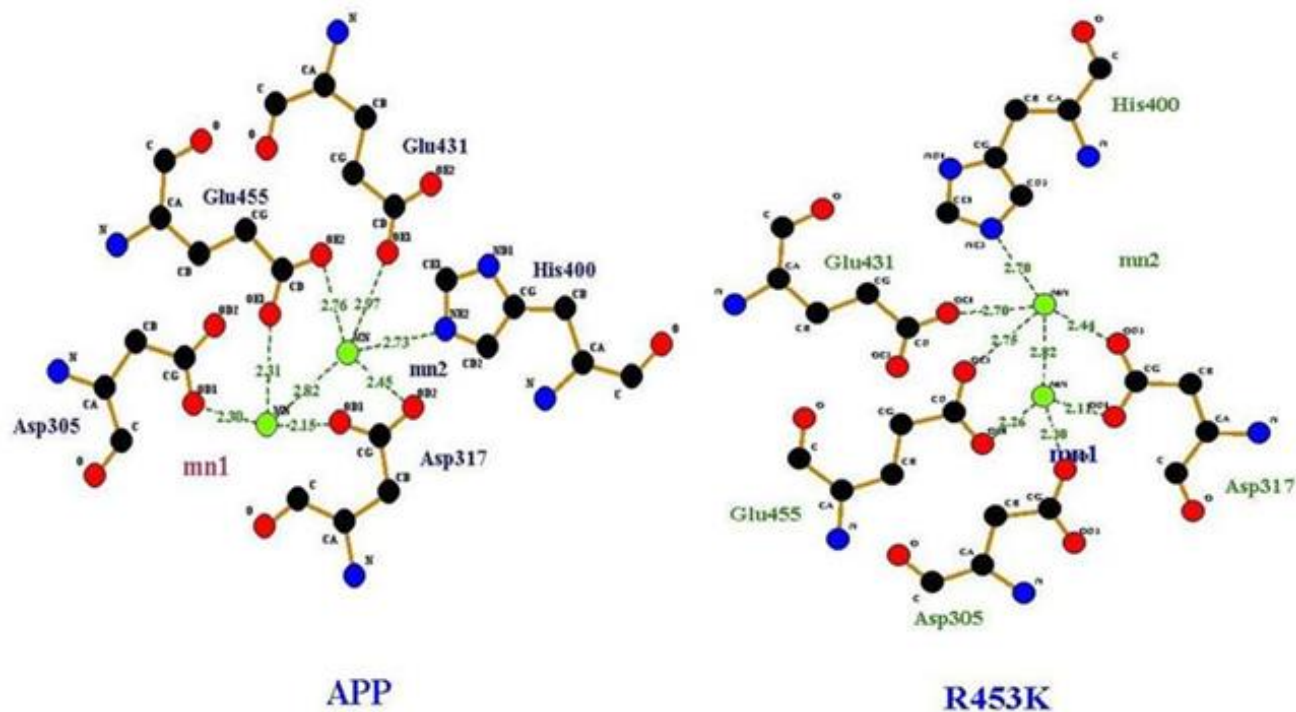
Figure 8. LigPlot representation of APP and APP mutant (R453K). The Mn^{2+} ions are represented by green spheres. Hydrogen bond interactions are represented by green dashed lines.
