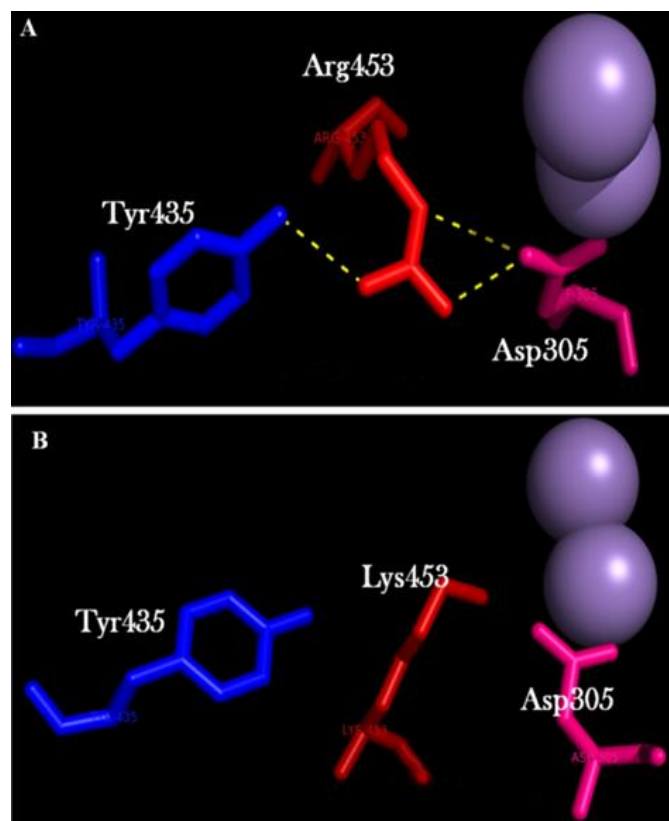
Figure 7. Comparison of the orientation of the hydrogen bond network in the active site of APP formed by Asp305, Arg453 and Tyr435. (A) The guanidinium group of Arg453 interacting with the carboxylate of Asp305 and the hydroxyl group of Tyr435 in the wild-type APP (B) the modeled structure displaying the relative position of R453K, showing the absence of hydrogen bond interactions with two neighboring residues. The hydrogen bonding interactions are shown as dashed yellow lines.
