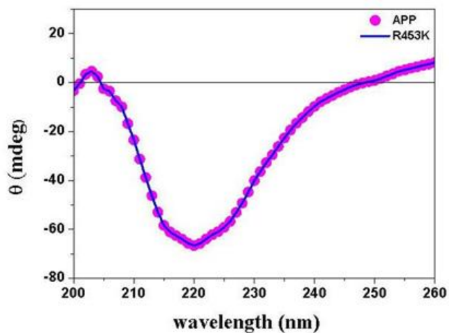
Figure 4. CD spectra of APP and R453K mutant.
