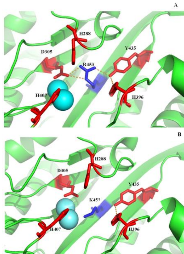
Figure 6. Comparison of active site organization of APP and R453K mutant protein. The active site of S. lavendulae APP (A) wild type (B) mutant R453K. The mutated residue is shown in blue.
