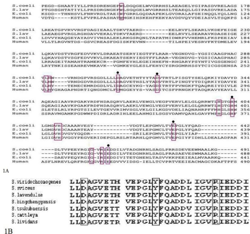
Figure 1. (A) Alignment of entire ORF sequences of APPs from S. coelicolor , S. lavendulae , E. coli and human. Multiple sequence alignments were performed using the CLUSTAL algorithm. The amino acid residues involved in catalysis are marked by boxes and those involved in metal coordination are indicated by black dots. (B) Aligned APP sequences of various Streptomyces stains. Conserved residues of interest Asp (D), Tyr (Y) and Arg (R) described are indicated in boxes.
