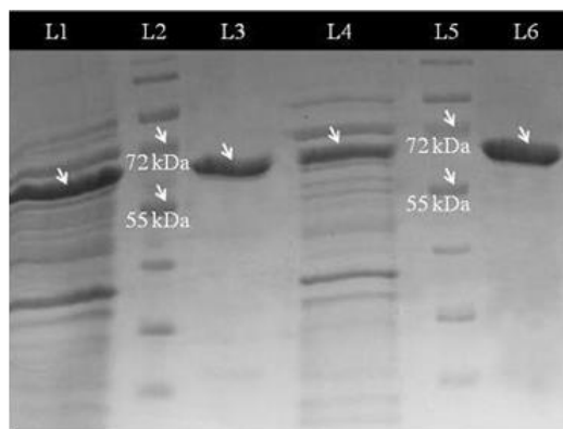
Figure 2. SDS-PAGE showing protein expression. L2 and L5- Protein markers; L1- APP overexpression; L3- Purified APP; L4- R453K overexpression; L6- Purified R453K.
