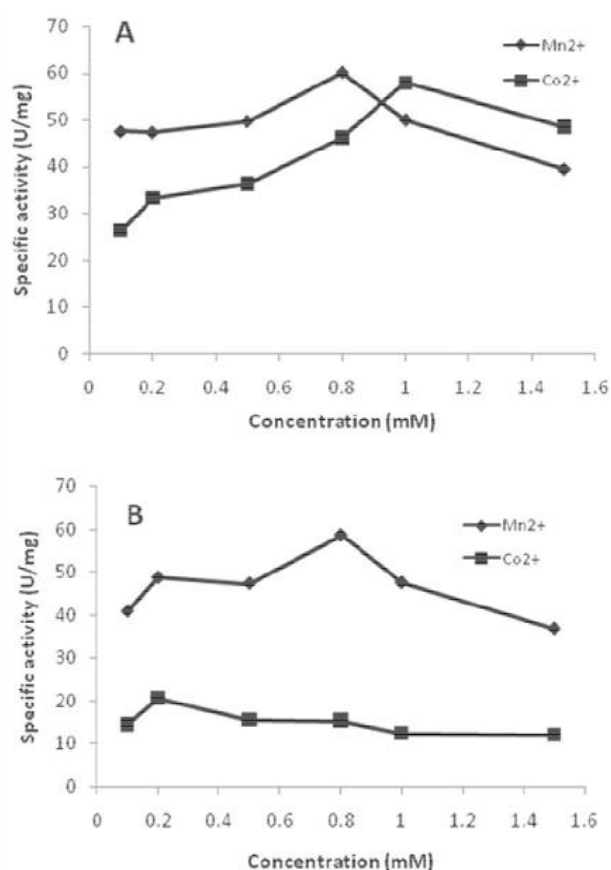
Figure 3. Effect of Mn^{2+} and Co^{2+} on enzyme activity (A) APP (B) in R453K mutant.
