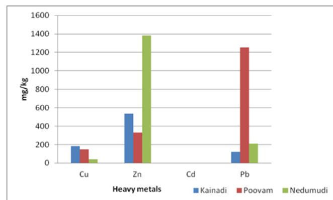
Figure 1. Heavy metals concentrations in the sediment samples
