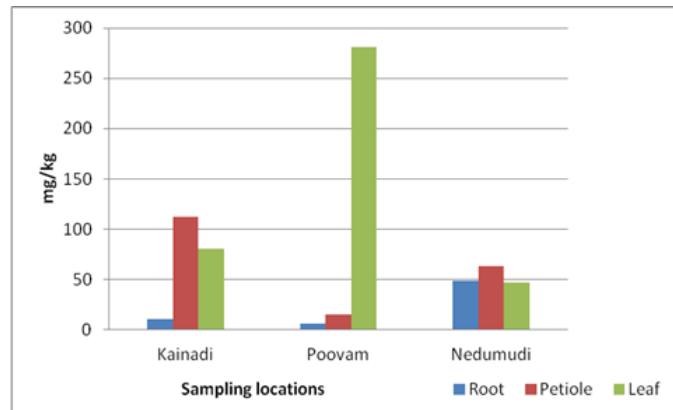
Figure 5. Lead accumulation in plant parts of Nymphaea pubescens
