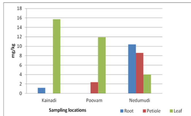
Figure 2. Copper accumulation in plant parts of Nymphaea pubescens
