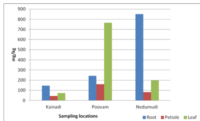
Figure 3. Zinc accumulation in plant parts of Nymphaea pubescens
