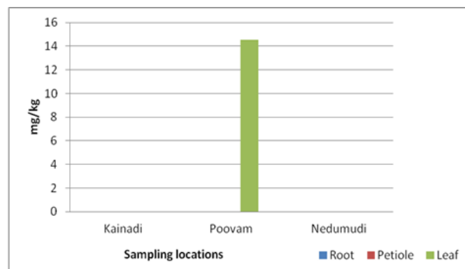
Figure 4. Cadmium accumulation in plant parts of Nymphaea pubescens
