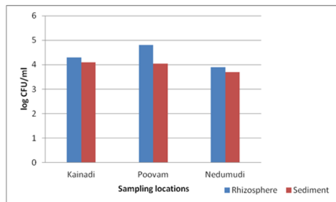
Figure 6. Load of rhizosphere and bulk sediment bacteria of Nymphaea pubescens
