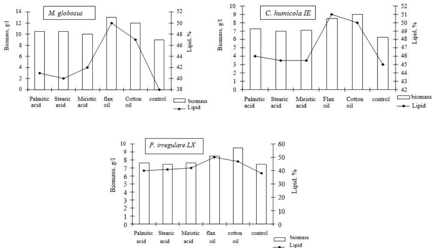
Figure 3. The effect of fatty acids and vegetable oils on growth and lipid production of fungi.
