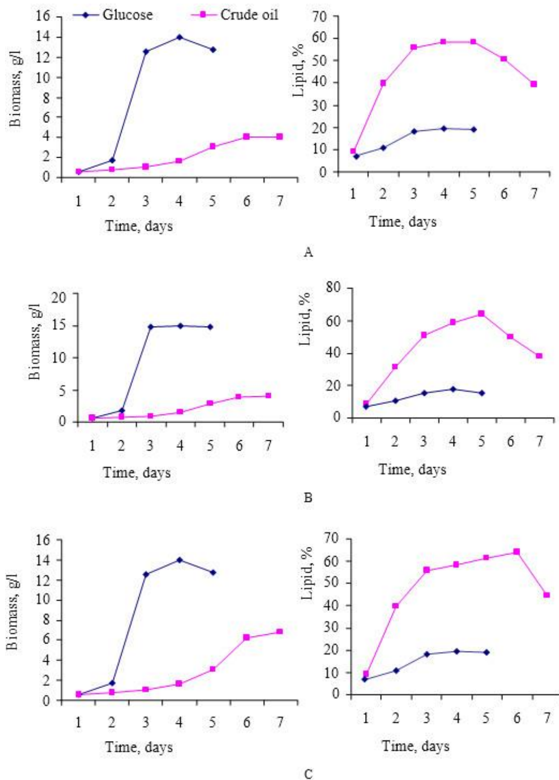
Figure 2. Growth and lipid accumulation in C. humicola IE (A), M. globosus 11 (B) and P. irregulare LX (C) grown on a medium with glucose and crude oil substrates.
