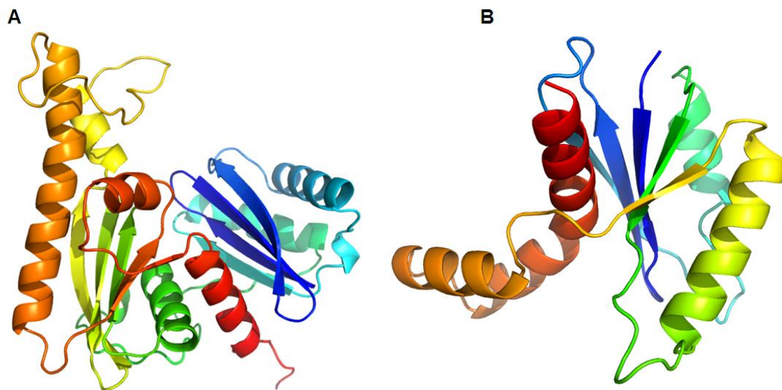
Figure 4. Generated model structures: A - Pantothenate kinase (LmPK) and B - Holliday junction resolvase like protein (LmHJR) of L. monocytogenes F2365.
