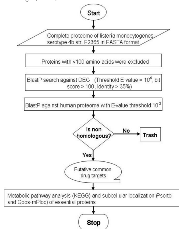
Figure 1. A flow chart describing the detailed methodology for identification of putative drug targets using subtractive genomics approach.
