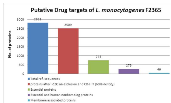
Figure 2. A chart showing putative drug targets of L. monocytogenes F2365 after several subsequent filtering steps.
