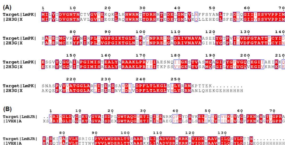
Figure 3. Sequence alignment of target proteins with their template sequences (A) - LmPK and template structure 2H3G_X (B) - LmHJR and its template structure 1VHX_A.
