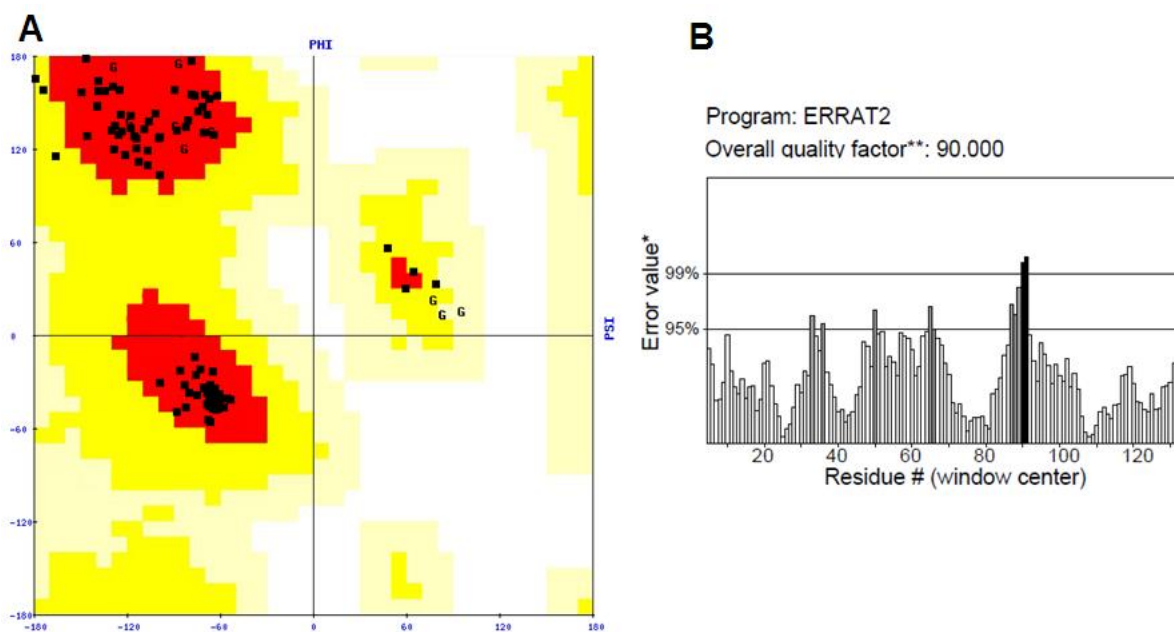
Figure 5. Ramachandran plot and overall quality factor of LmHJR model computed using Procheck ( A ) and ERRAT2 ( B ) program.
